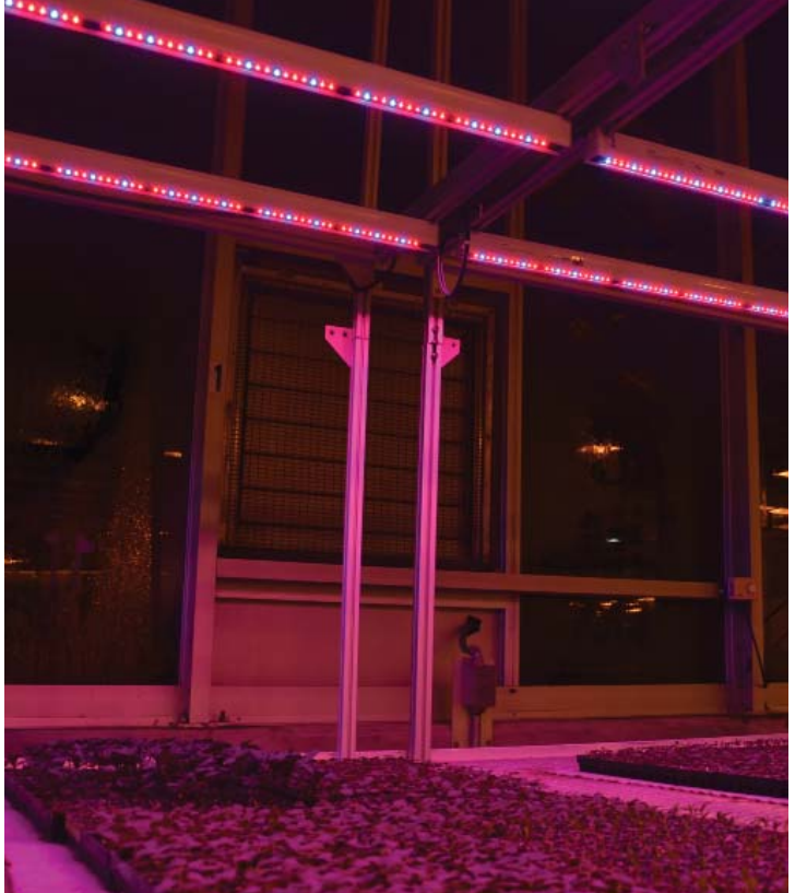
Figure 2. Greenhouse supplemental lighting of bedding plant plugs using LEDs delivering 70 \mu\text{mol}\cdot\text{m}^{-2}\cdot\text{s}^{-1} of (%) 87:13 red:blue light at canopy level.
