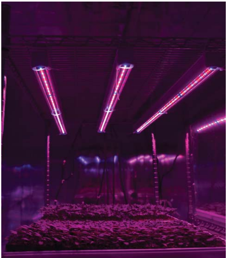
Figure 3. Multi-layer, sole-source indoor production of plugs using LEDs delivering 185 \mu\text{mol}\cdot\text{m}^{-2}\cdot\text{s}^{-1} of (%) 88:12 or 70:30 (not shown) red:blue light at canopy level.
